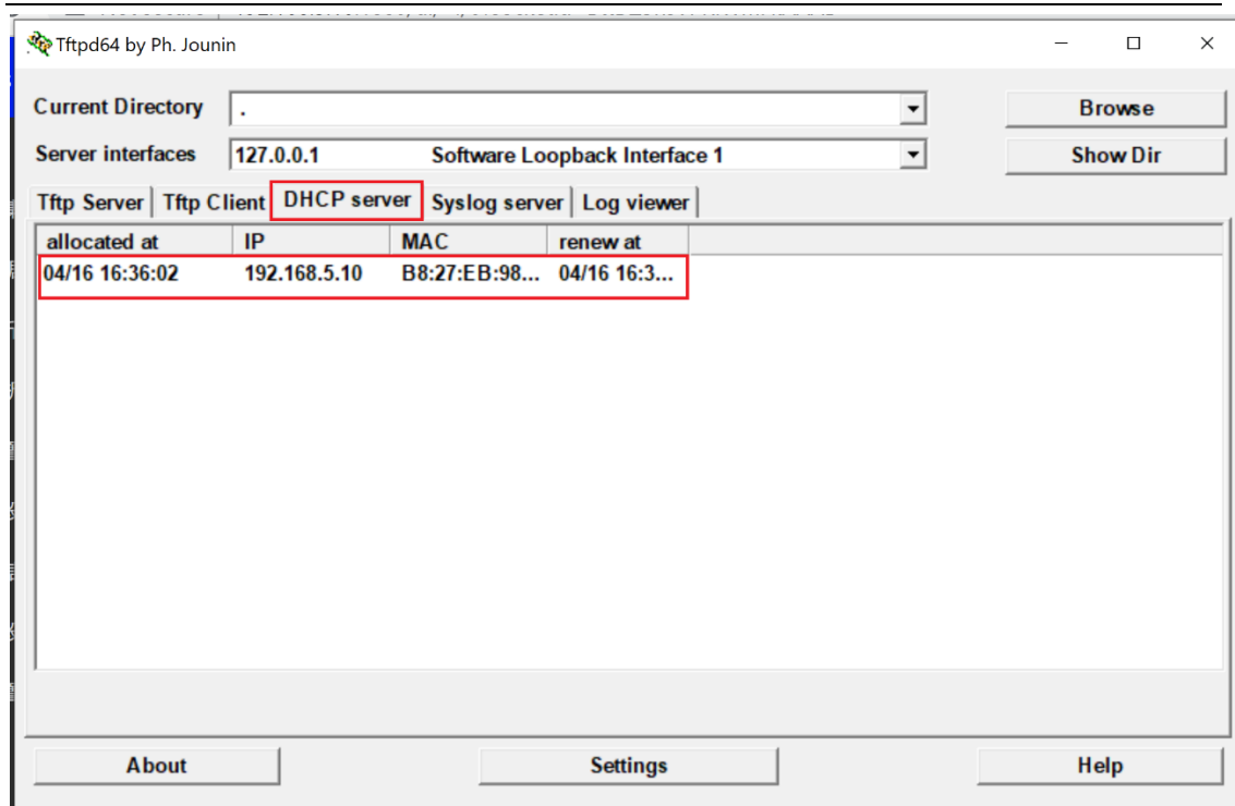
Figure 117 Find new IP for gateway
