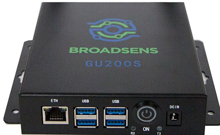
Figure 2 GU200S connectors
