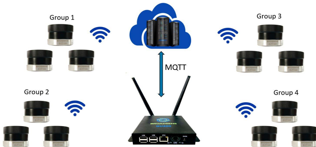
Figure 1 Group control of multiple wireless sensors
