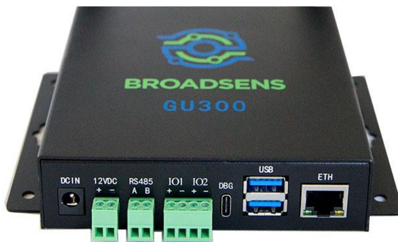
Figure 3 GU300 connectors
