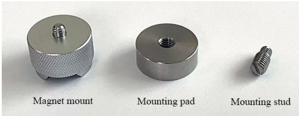
Figure 19 Vibration sensor mounting
