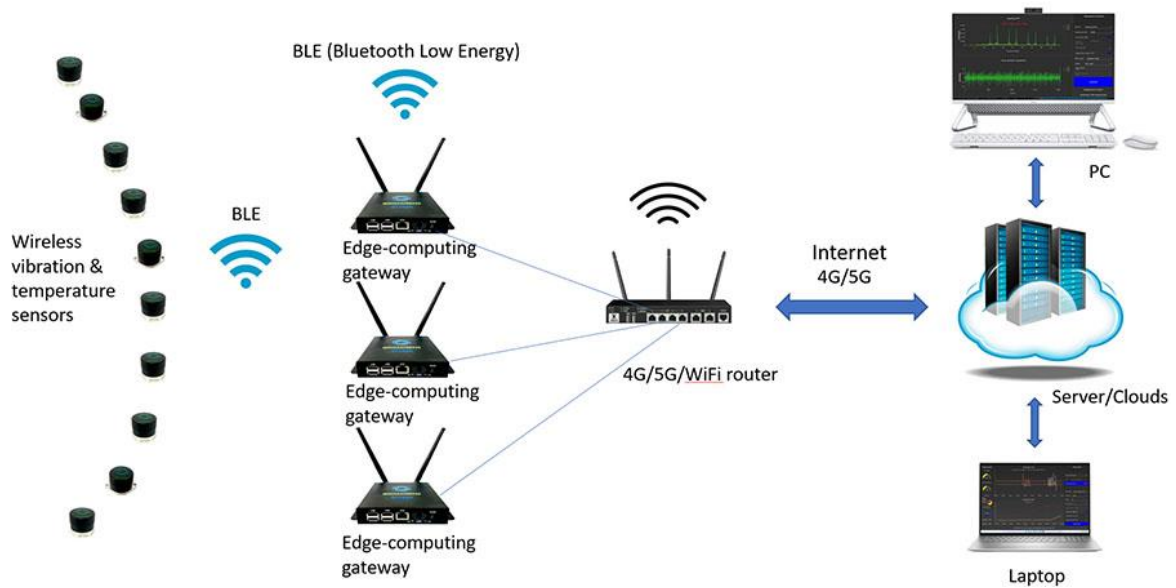
Figure 5 System connection
