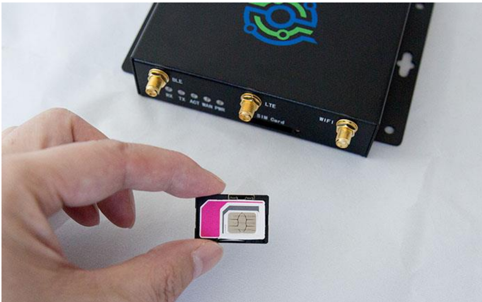
Figure 10 Insert SIM card to the SIM card tray
