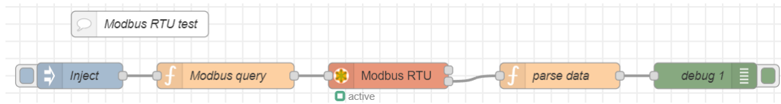
Figure 101 Modbus RTU test flow
