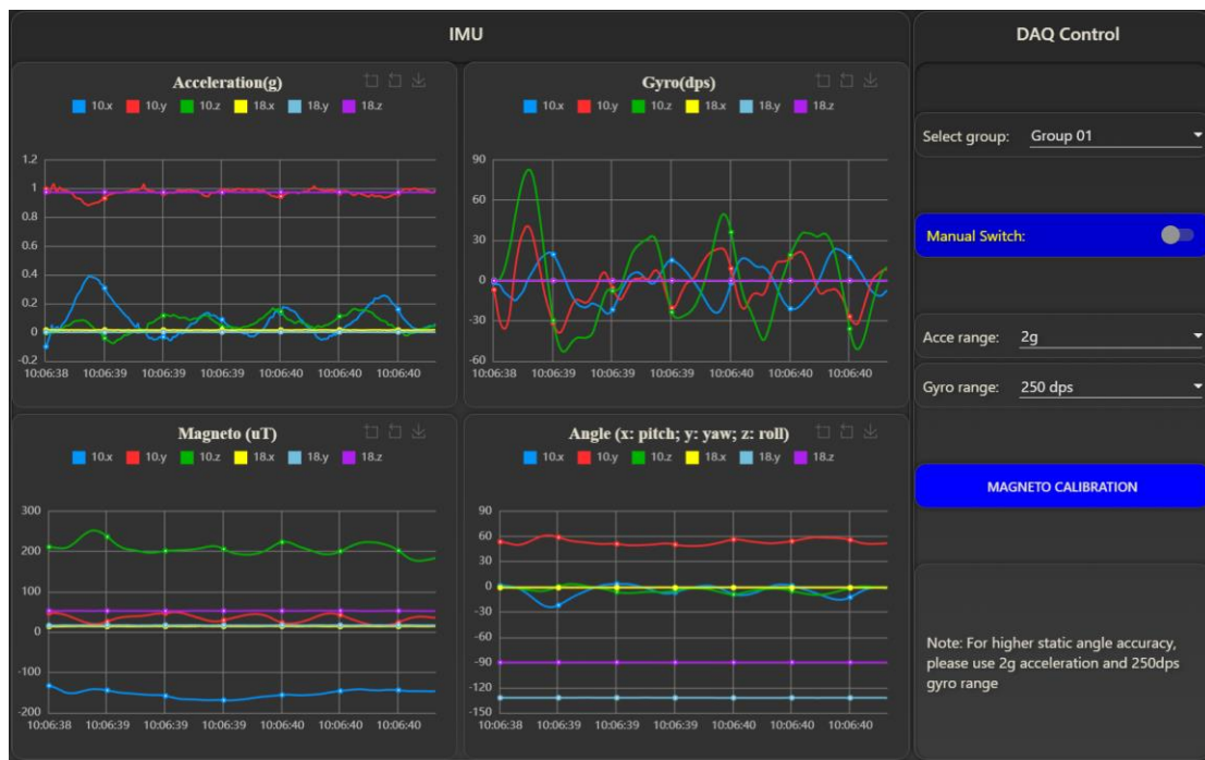
Figure 104 SAG IMU sensor DAQ
