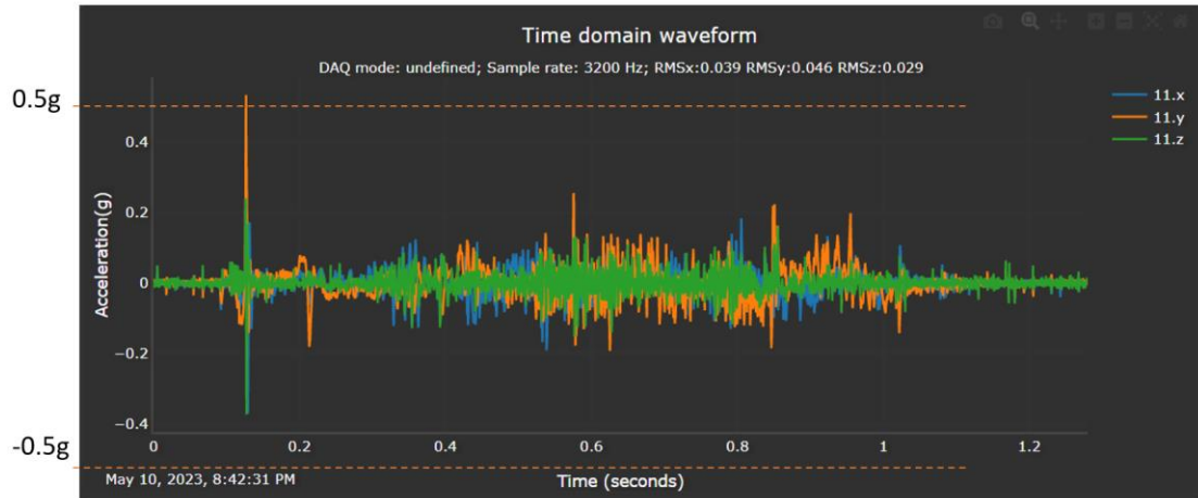
Figure 39 Shock event captured by defining a trigger threshold
