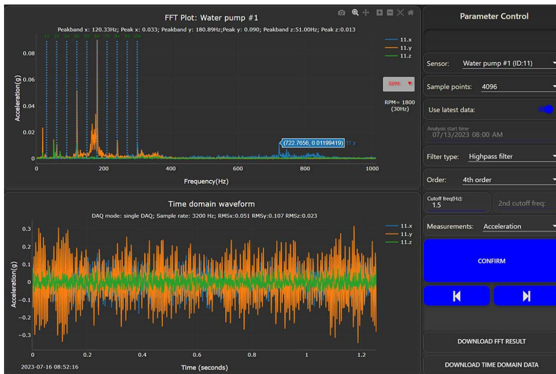
Figure 59 FFT analysis
